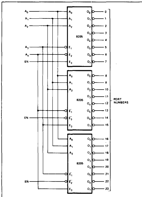
Figure 4. I/O Port Decoder
