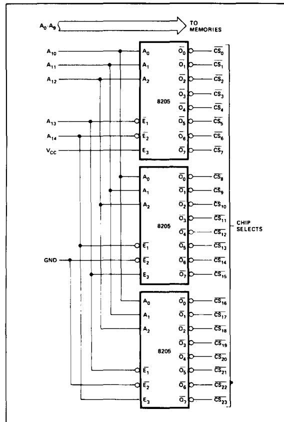
Figure 5. 24K Memory Interface
