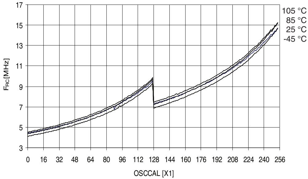
Figure 31-354.ATmega3250PA: Calibrated 8MHz RC Oscillator Frequency vs. Oscscal Value
